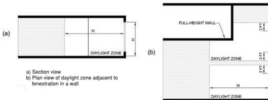
FIGURE C405.2.3.2 SIDELIT ZONE
