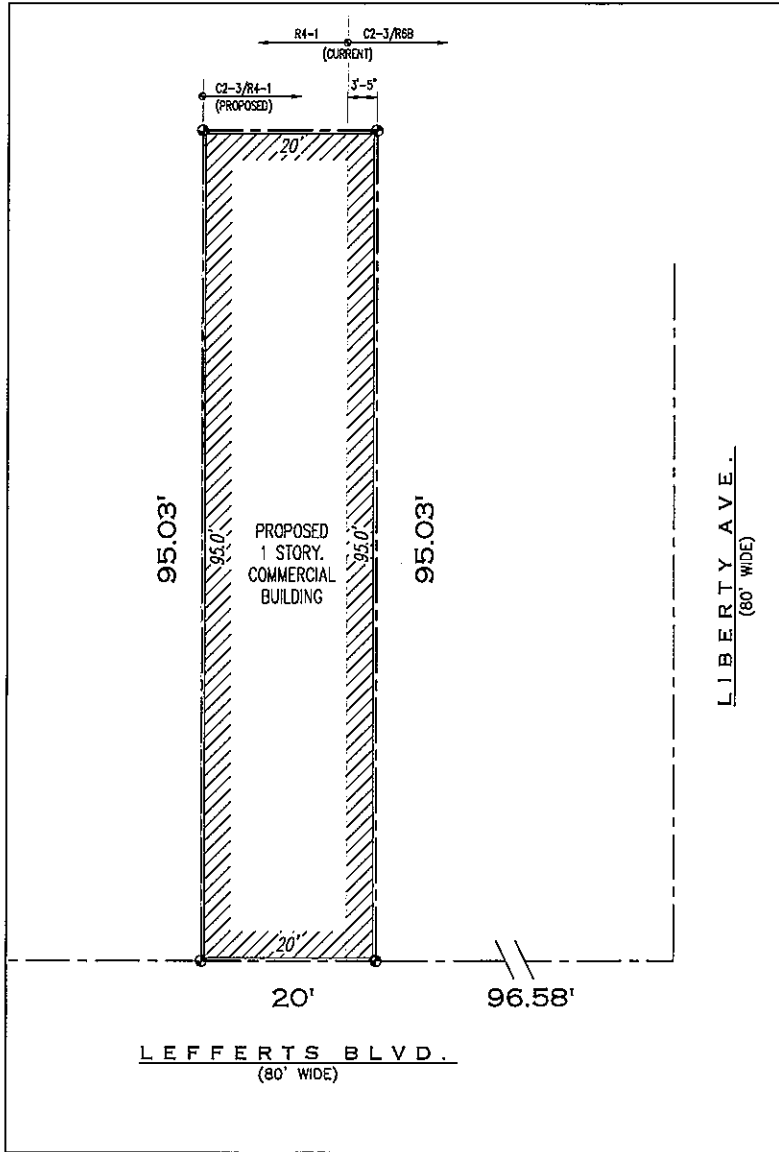
PLOT PLAN SCALE: 1" = 10'
