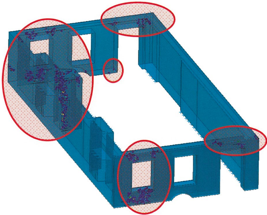
PREDICTED DAMAGE AT EXTERIOR WALLS
