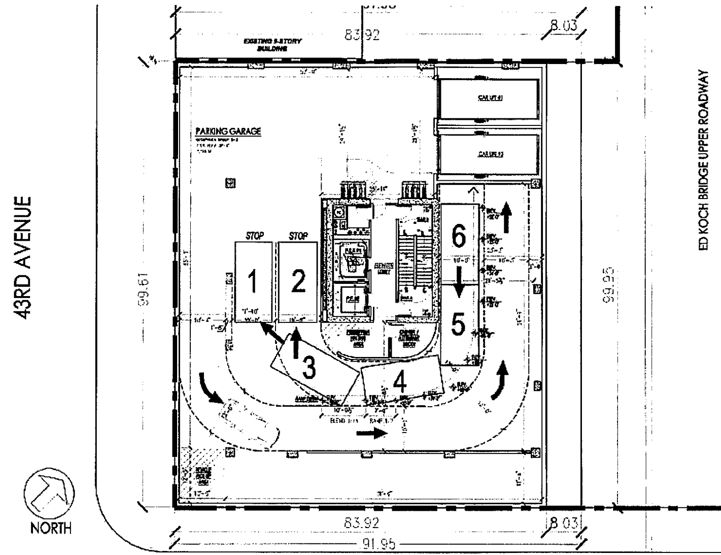
2nd Floor Parking Plan
