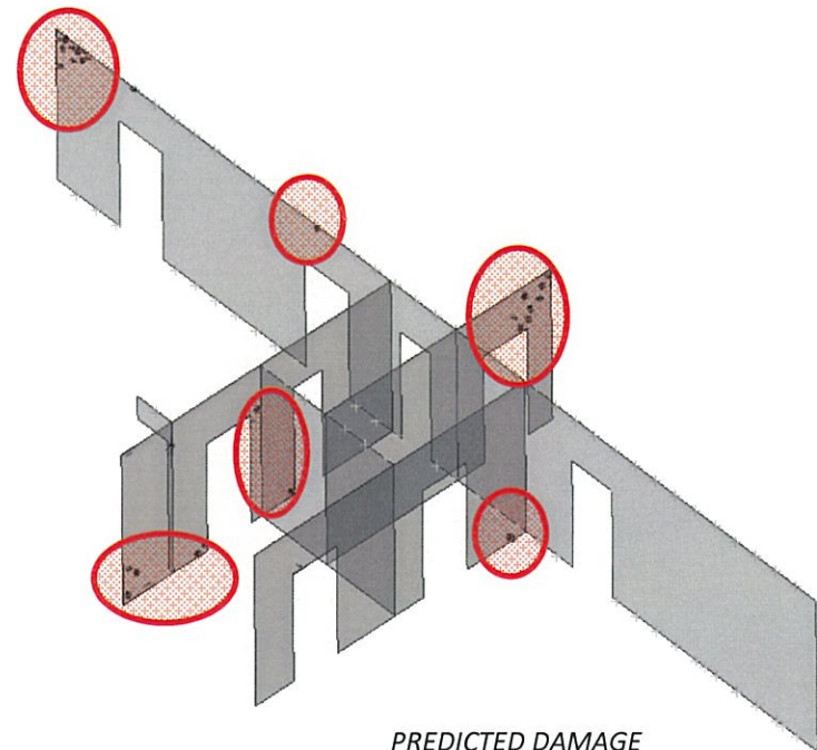
PREDICTED DAMAGE AT INTERIOR WALLS
