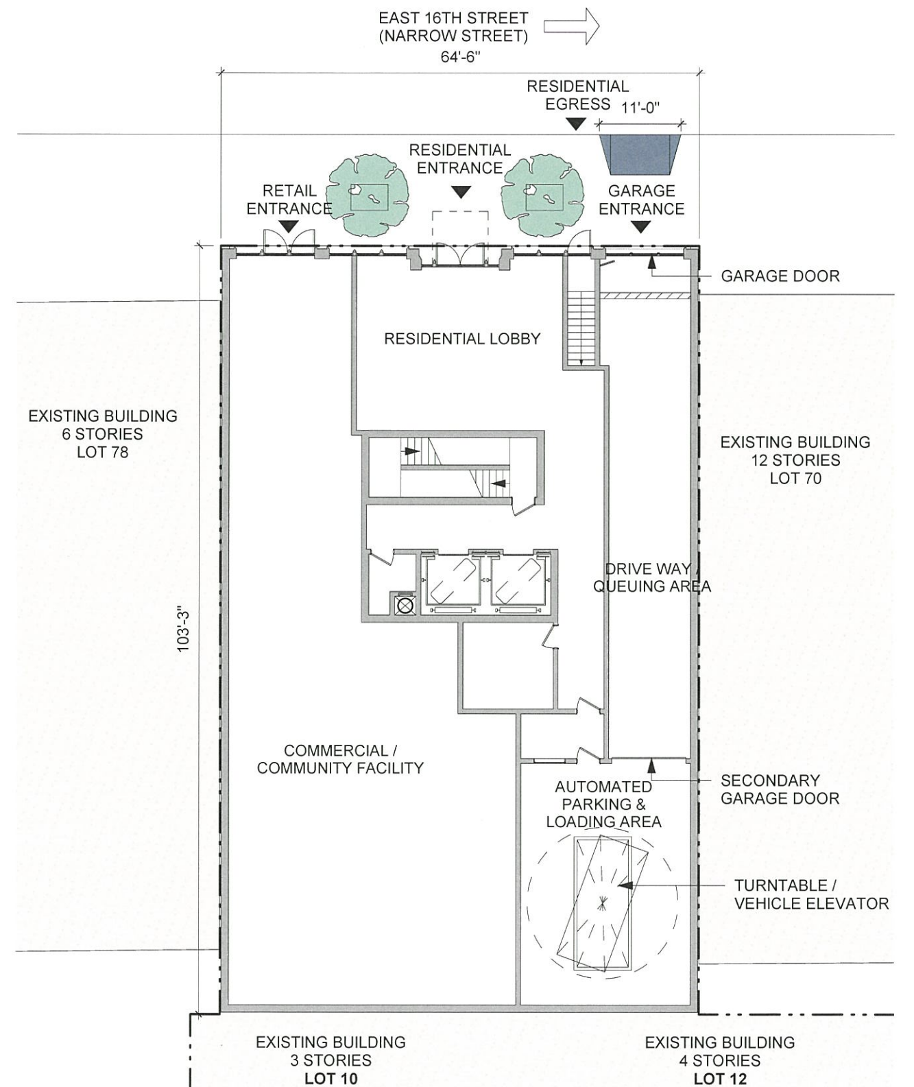
PROPOSED BUILDING
