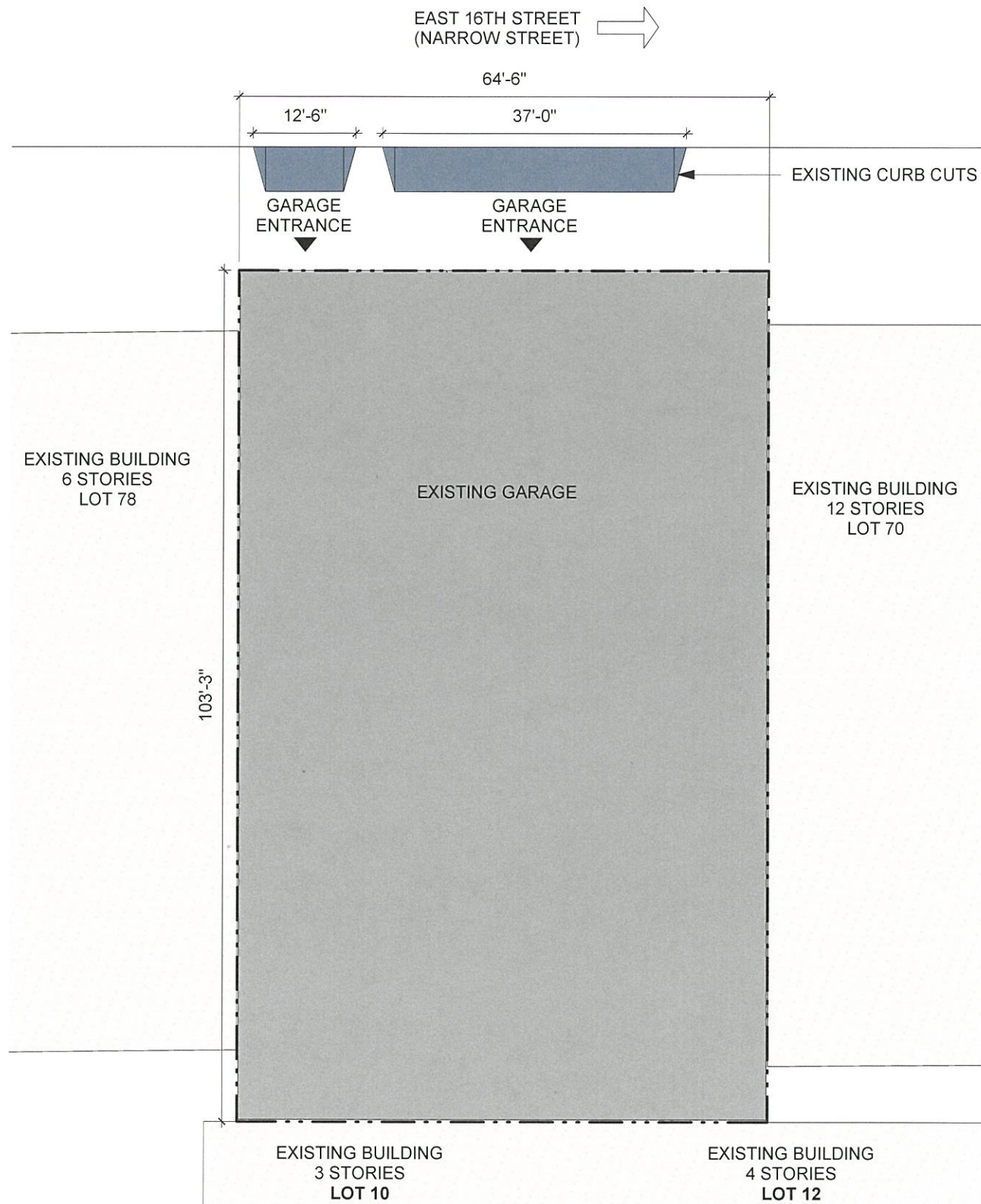
EXISTING CONDITIONS
