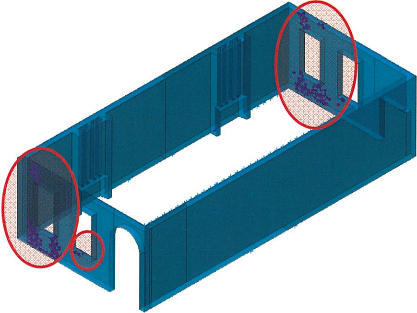
PREDICTED DAMAGE AT EXTERIOR WALLS
