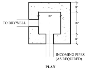
FIGURE 1114.2.3(1) YARD DRAIN WITH SUMP
